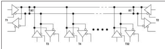
Typical RS485 application multi point network
