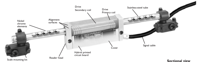
Sectional view
