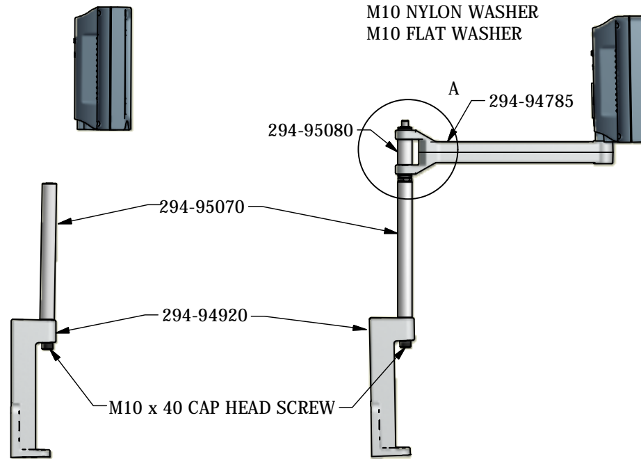
CARRIAGE ADAPTOR ASSY WITH EXTENSION ARM
